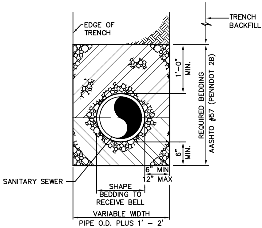
D.I. PIPE EMBEDMENT
